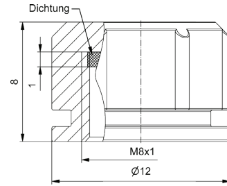
Dimension Male connector
