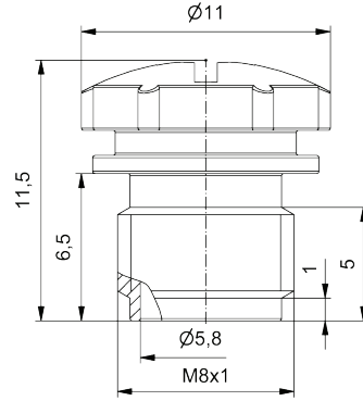
Dimension Female connector
